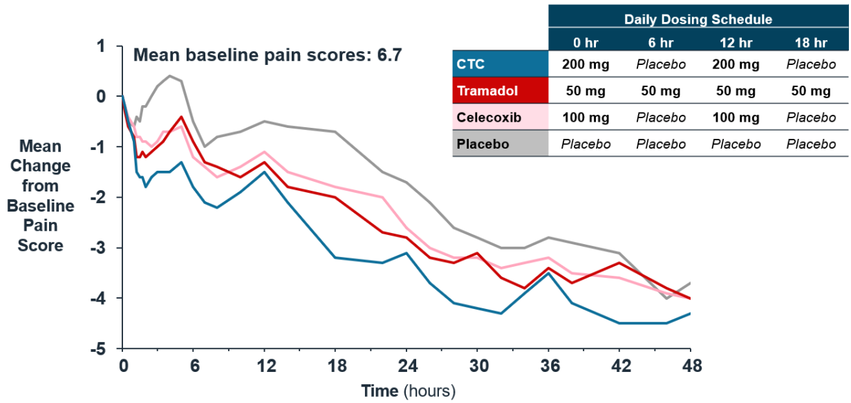
Figure 33: Pain Intensity Differences Over Time (FAS) in Study 301
